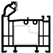
72MM PVC-U THRESHOLD (OVOLO)
