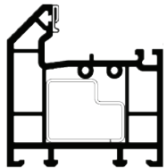
72MM PVC-U THRESHOLD (BEVELLED)
