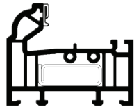
56MM PVC-U THRESHOLD (OVOLO)
